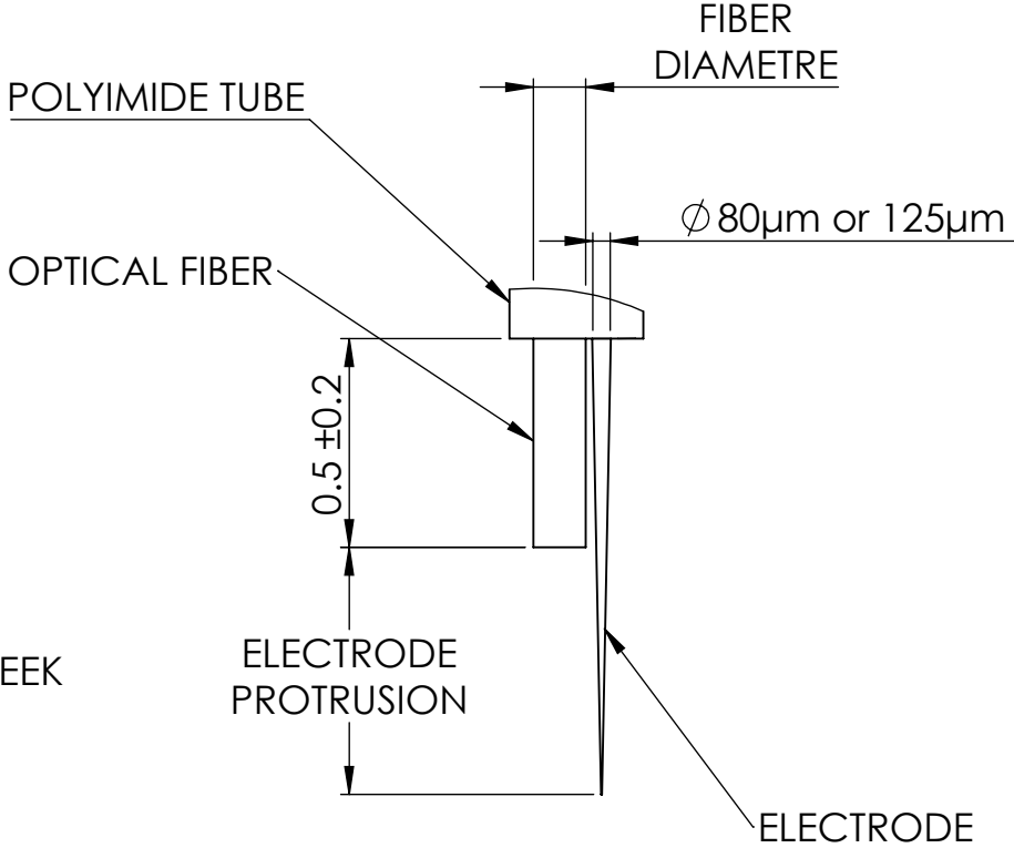
DETAIL FIBER TERMINATION SCALE 50 : 1
